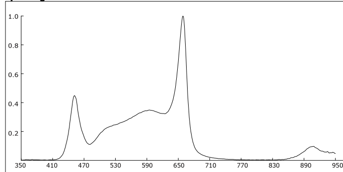
Spectrogram
