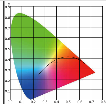
CIE1931
