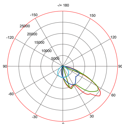
Chart 2: Isocandela Plot AVERAGE BEAM ANGLE(50%): 71.2 DEG
